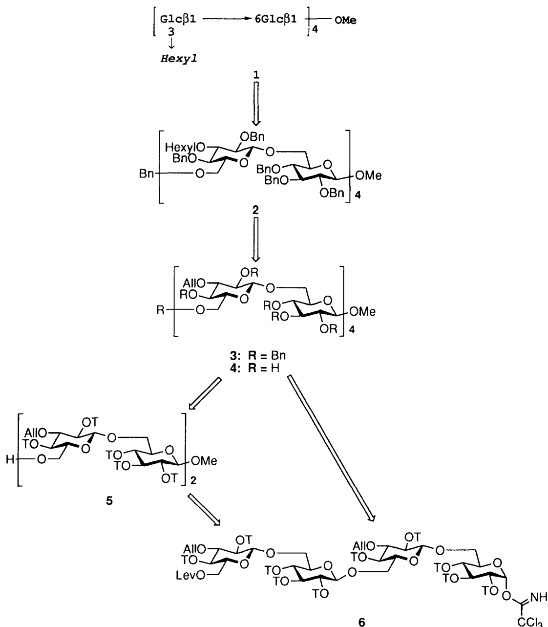
Figure 3. Synthetic strategy.
